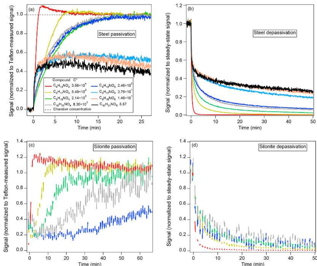
Figure 4. Examples of passivation and depassivation of stainless steel (a, b) for C_6 – C_{10} HN and DHN and Silonite (c, d) for C^* > 10^2 \mu\text{g m}^{-3} HN and DHN, where curves were binomially smoothed across 10 points for visual clarity. The stainless-steel data were measured by the CU (Ziemann) CIMS. The Silonite data were measured with the UW CIMS, and the gaps were due to periodic background sampling. Note that the starting signals for (c) are not zero, due to compounds that remained in the instrument.
