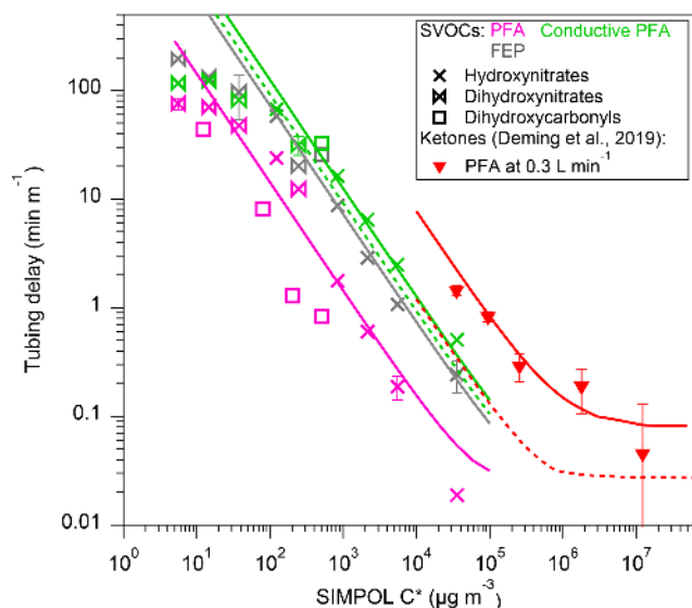
Figure 3. Measured tubing delays normalized by tubing length as a function of the saturation concentration of the gas compounds. Also shown as a comparison is the PFA result by Deming et al. (2019). Example error bars are shown, as propagated from exponential fits. Solid lines are chromatographic model results using the best estimated C_w (for C^* = 10^2 – 3 \times 10^4 \mu\text{g m}^{-3} ) for different tubing at the same flow rates (Table 1). Dashed lines are model results for conductive PFA (this study) and PFA (Deming et al., 2019), using the C_w determined in that work at 4 \text{ L min}^{-1} .
