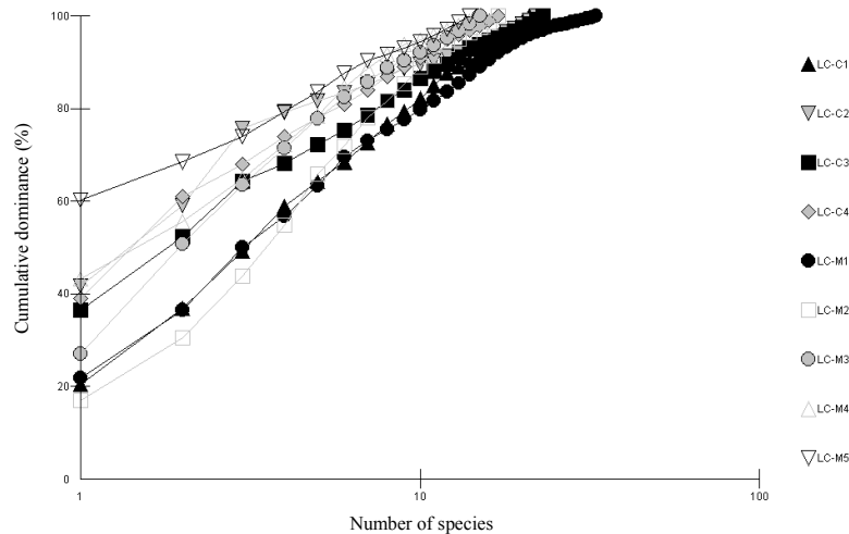
Fig. 7. Dominance curves of sampling stations.
