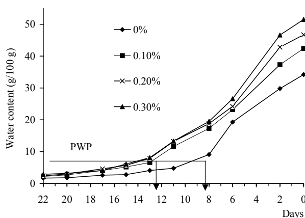
Figure 4. Effects of hydrogel concentration on water storage of loam soil; PWP refers to permanent wilting point and the arrows indicate the days for onset of PWP at different hydrogel levels
