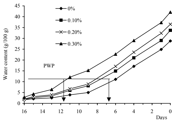
Figure 3. Effects of hydrogel concentration on water storage of sandy loam soil; PWP refers to permanent wilting point and the arrows indicate the days for onset of PWP at different hydrogel levels
