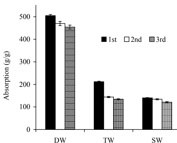
Figure 1. Absorption of distilled water (DW), tap water (TW) and saline water (SW) by gel during 1 st , 2 nd and 3 rd wetting and drying cycle
