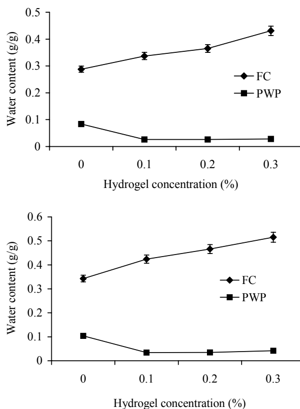
Figure 2. Effects of hydrogel levels on water content at field capacity and permanent wilting point in sandy loam (above) and loam (below) soils; the difference between water content at field capacity and permanent wilting point shows the total plant available water
