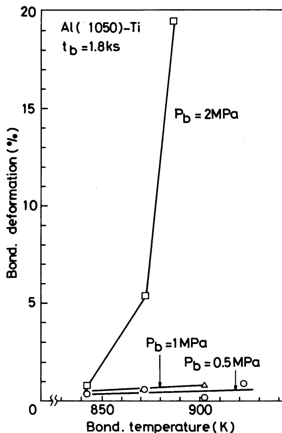
Fig. 6 Deformation of aluminum specimen \delta (%) vs. welding temperature for the diffusion-welded joint of titanium to 1050.
