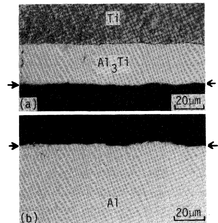
Fig. 9 Cross-sectional microstructures of a fractured zone in a joint of titanium to 4N aluminum fractured at the bond interface on tensile test: (a) titanium side and (b) aluminum side ( T_b = 923 K, P_b = 0.5 MPa and t_b = 1.8 ks). The arrows on both sides of the photographs indicate the fractured surfaces.
