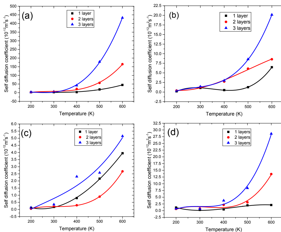
Figure 10: Diffusion coefficient of inorganic cations after salts addition; \text{NH}_4^+ (a), Mg (b); Al (c), and Fe (d) cations.
