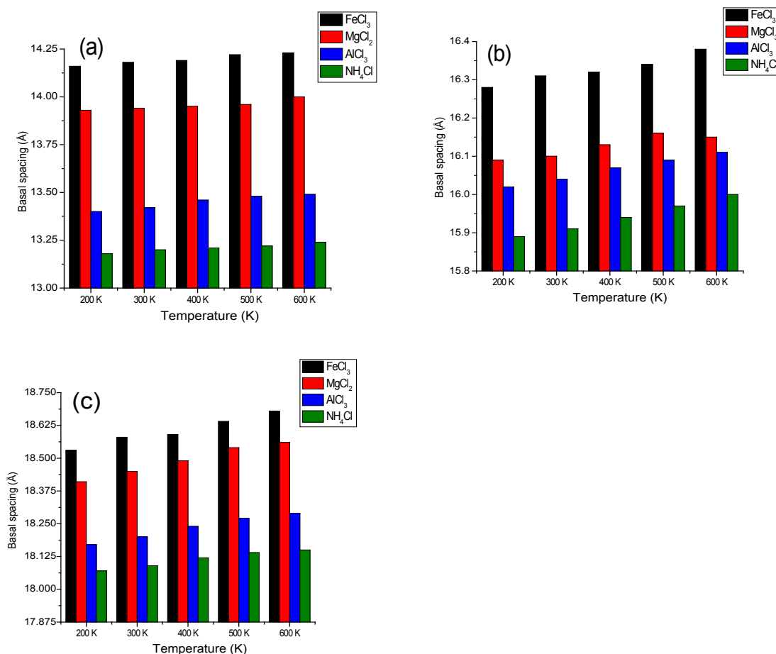
Figure 14: Basal spacing changes with respect to temperature for different layered Na-Mt after adding inorganic salts; (a), (b), (c) represent 1-, 2-, and 3 hydration layers respectively.
