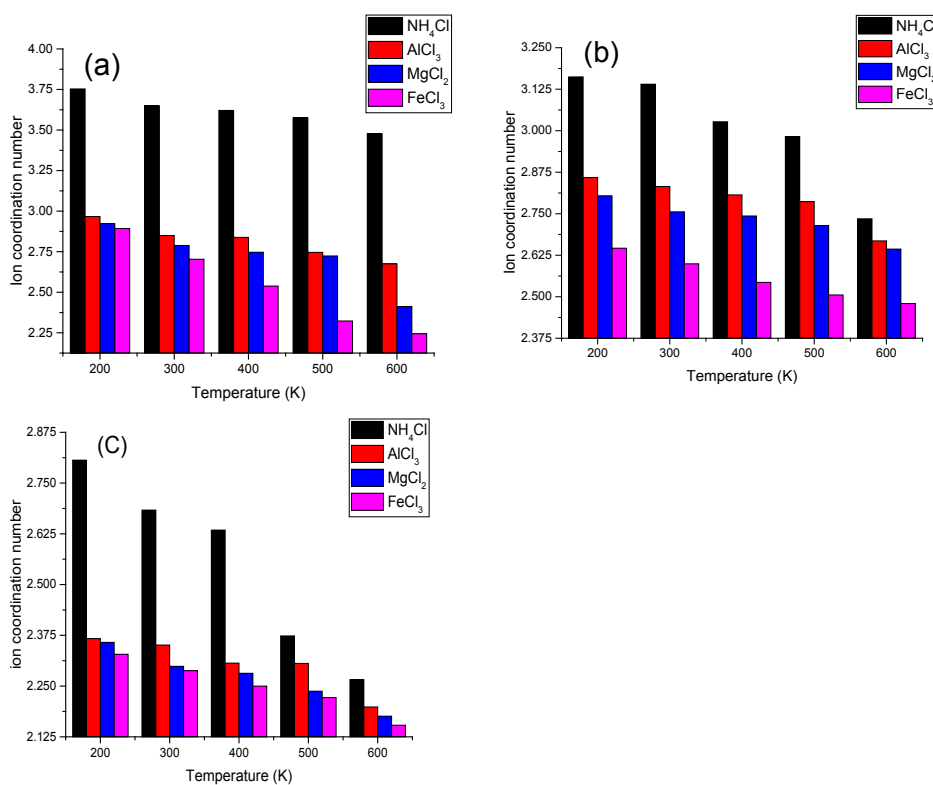
Figure 7: Ion coordination number of Cl anions after inorganic salts addition; (a), (b), (c) represent 1-, 2-, and 3 hydration layers respectively.
