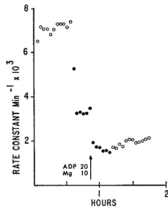
FIGURE 7. Effect of injected ADP + Mg (2:1) on sodium efflux from squid axon. Open circles, 9 mM K_o ; filled circles, 0 mM K_o . Arrow indicates time when ADP + Mg was injected to give approximately the final concentrations indicated. Axon 40568. Diameter 425 \mu . Temperature 11°C.
