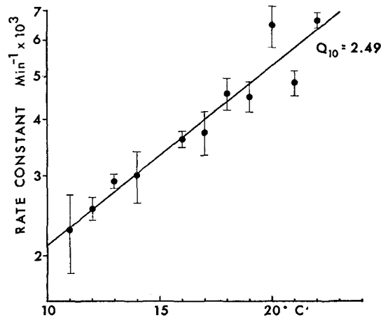
FIGURE 1. Temperature dependence of sodium efflux from squid giant axon. Data from 115 axons. For any given temperature, rate constants for individual axons were normalized to a diameter of 500 \mu , and pooled. The points shown are means (from 3–27 axons) \pm SE. The curve, fitted by a least squares procedure to the unweighted means, obeys equation: \text{Log} [\text{rate constant (in min}^{-1}) \times 10^3] = -0.07174 + 0.3966 \text{ temperature } (^\circ\text{C}) corresponding to a temperature coefficient Q_{10} = 2.49 .
