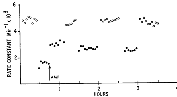
FIGURE 8. Effect of injected AMP on K sensitivity of sodium efflux from squid axon. Open circles, 9 mM K_o ; filled circles, 0 mM K_o . Arrow indicates time of injection of AMP to make a final concentration of 20 mM. Axon 81068B. Diameter 490 \mu . Temperature 18°C.
