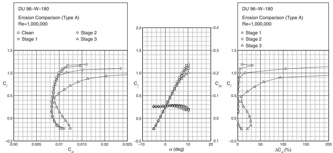
Figure 6. Effect of Type A leading edge erosion on the performance of the DU 96-W-180 airfoil and the resulting percentage increase in drag at Re = 1,000,000 .
