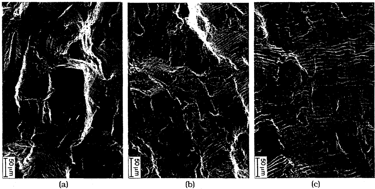
Figure 5. Photomicrographs of fracture surface of Type 316NG SS specimens tested at 288°C in (a) air, (b) high-DO water, and (c) simulated PWR water
