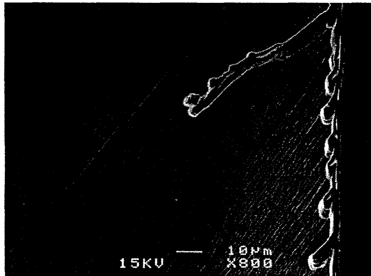
Figure 6. Photomicrographs of surface cracks along longitudinal sections of Type 316 NG stainless steel tested at 288°C in low- and high-DO water
