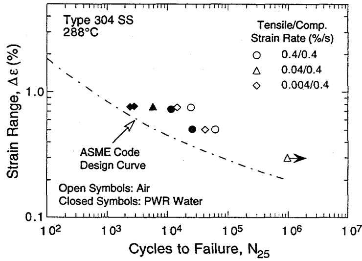
Figure 3. Total strain-range-vs.-fatigue-life data for Types 316 NG and 304 SS in air and water
