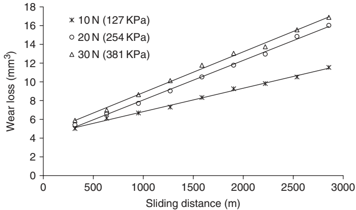
Figure 2. Effect of sliding distance and contact load on wear loss of unfilled epoxy.
