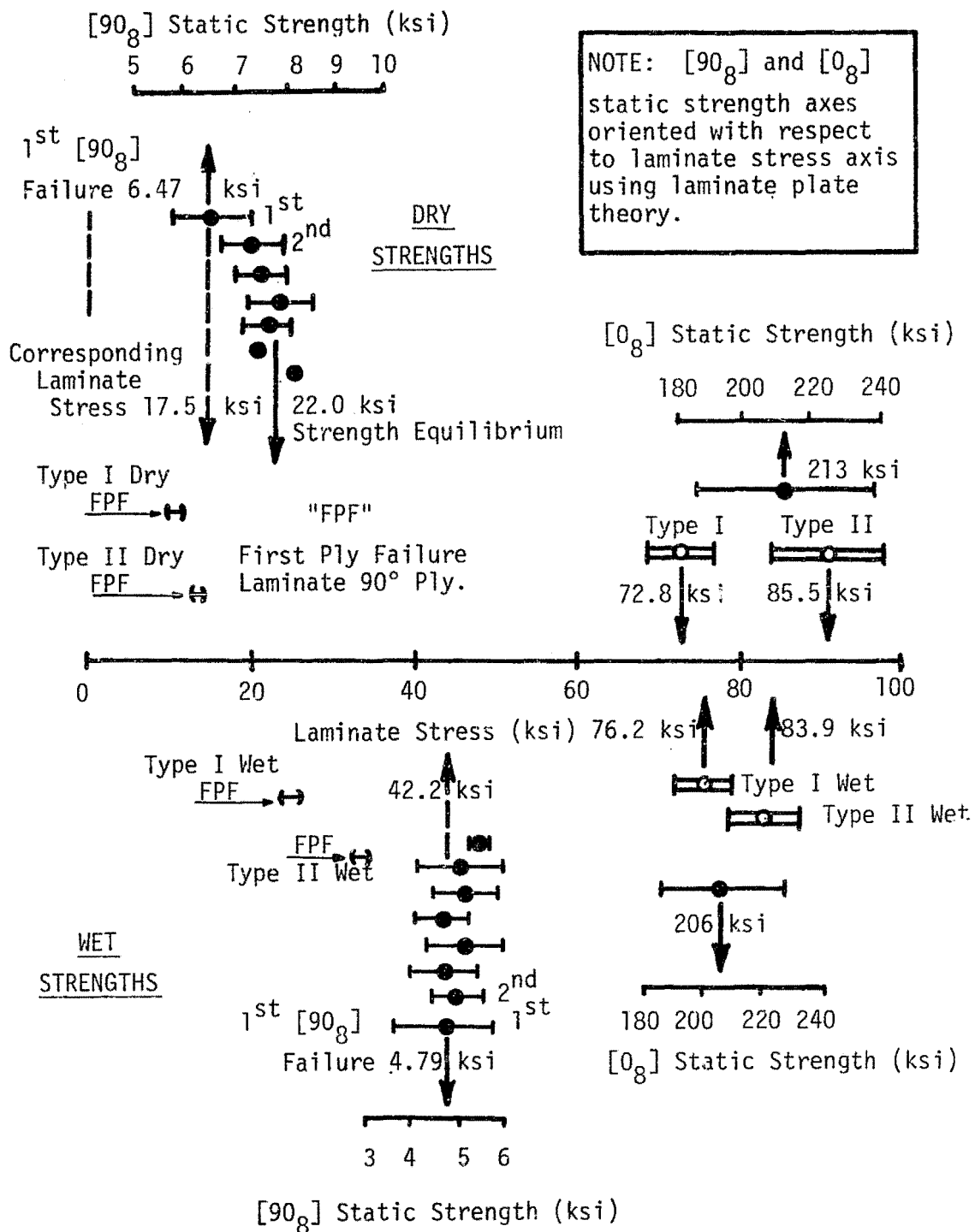
FIGURE 16. CORRELATION OF WET AND DRY [0_8] and [90_8] STATIC STRENGTHS WITH TYPE I AND TYPE II LAMINATE STRESS STATE AND FIRST 90^\circ PLY FAILURES.
