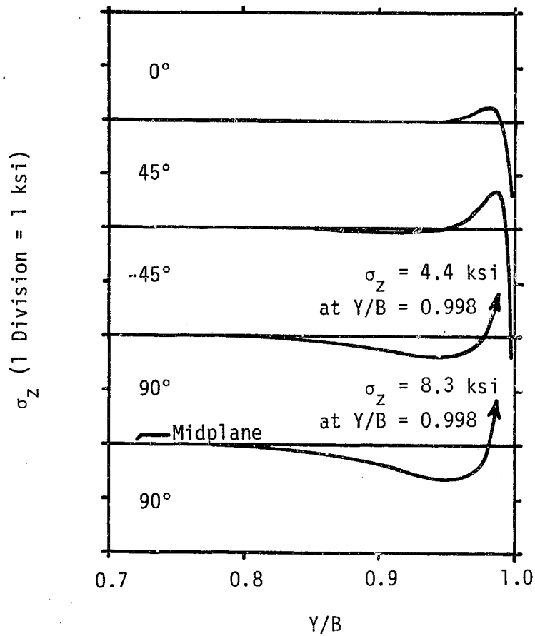
FIGURE 4. VARIATION OF \sigma_z NEAR THE FREE EDGE OF A TYPE I WET LAMINATE ( N_x = 1900 lb/in, \Delta T = -180^\circ\text{F} , \Delta M = 1.2\% )
