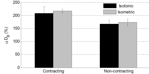
Fig. 5. Comparison of average DCS signals ( \alpha D_B ) [mean \pm SE, n = 10 (trials)] during isotonic and isometric exercises. Here the “Contracting” data during isotonic/isometric exercise represents the PF-120°/PF-90°, and “Non-contracting” represents the muscle in a relaxed state for both exercises. DCS data presented here are not influenced by any known motion artifacts, and therefore these signals are believed to originate from the muscle blood flow. Without motion artifacts the isotonic exercise produced similar level DCS flow signals compared to the isometric exercise, when the exercise intensity was set up at the same level (30% of highest MVIC) and the muscle worked in the same way (contracting or non-contracting).
