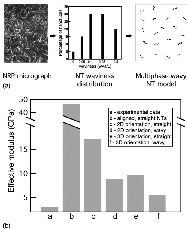
FIG. 3. (a) Schematic of the micromechanical approach to account for nanotube waviness. (b) Experimental data (10 wt% MWNTs in polystyrene) (Ref. 11) and micromechanical predictions (assuming straight and wavy nanotubes) of NRP effective moduli with different NT orientations. The modulus of the polystyrene matrix was 1.91 GPa, and the following parameters describe the discrete NT phases modeled in the wavy NT calculations: ( w=0 , E_{\text{wavy}}=450 GPa, NT fraction=0.05), (0.05, 377, 0.15), (0.1, 283, 0.30), (0.25, 91, 0.30), (0.5, 42, 0.20).
