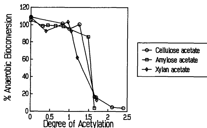
Fig. 6. A summation of the anaerobic bioconversion of the natural polymer acetylation series. Data represent the average of triplicate experimentals. Data represent a total incubation period of 90–98 d.
