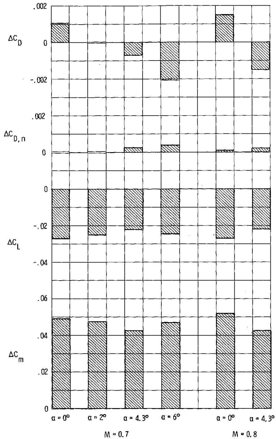
Figure 39.- Increments in afterbody-nozzle aerodynamic characteristics due to deflecting horizontal tails from 0^\circ to -2^\circ with type A cruise nozzles and interfering 2.
