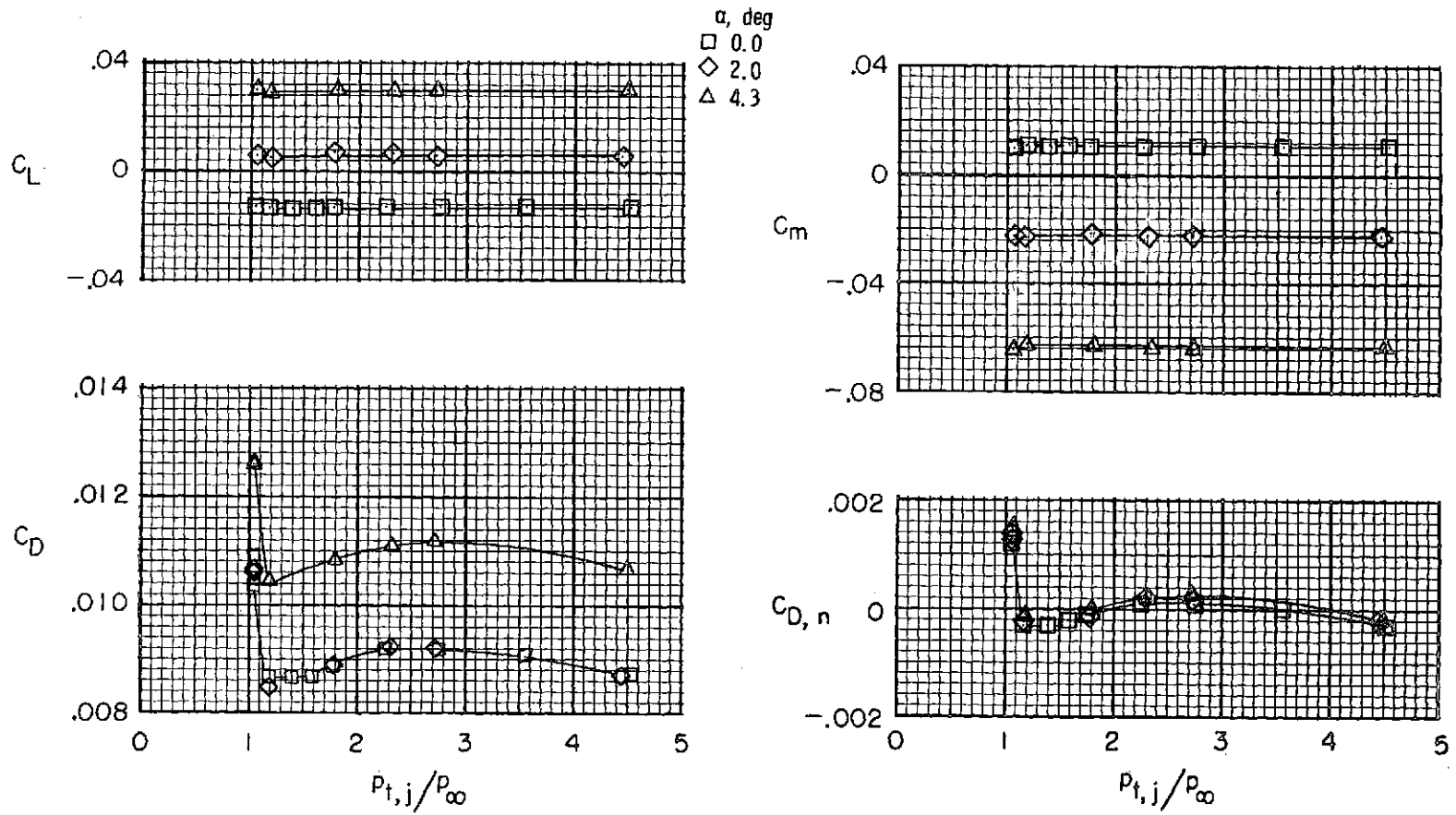
Figure 21.- Effect of jet total-pressure ratio on afterbody-nozzle aerodynamic forces and moments for type B cruise nozzles and interfering 5. Dashed line indicates possible fouling.
