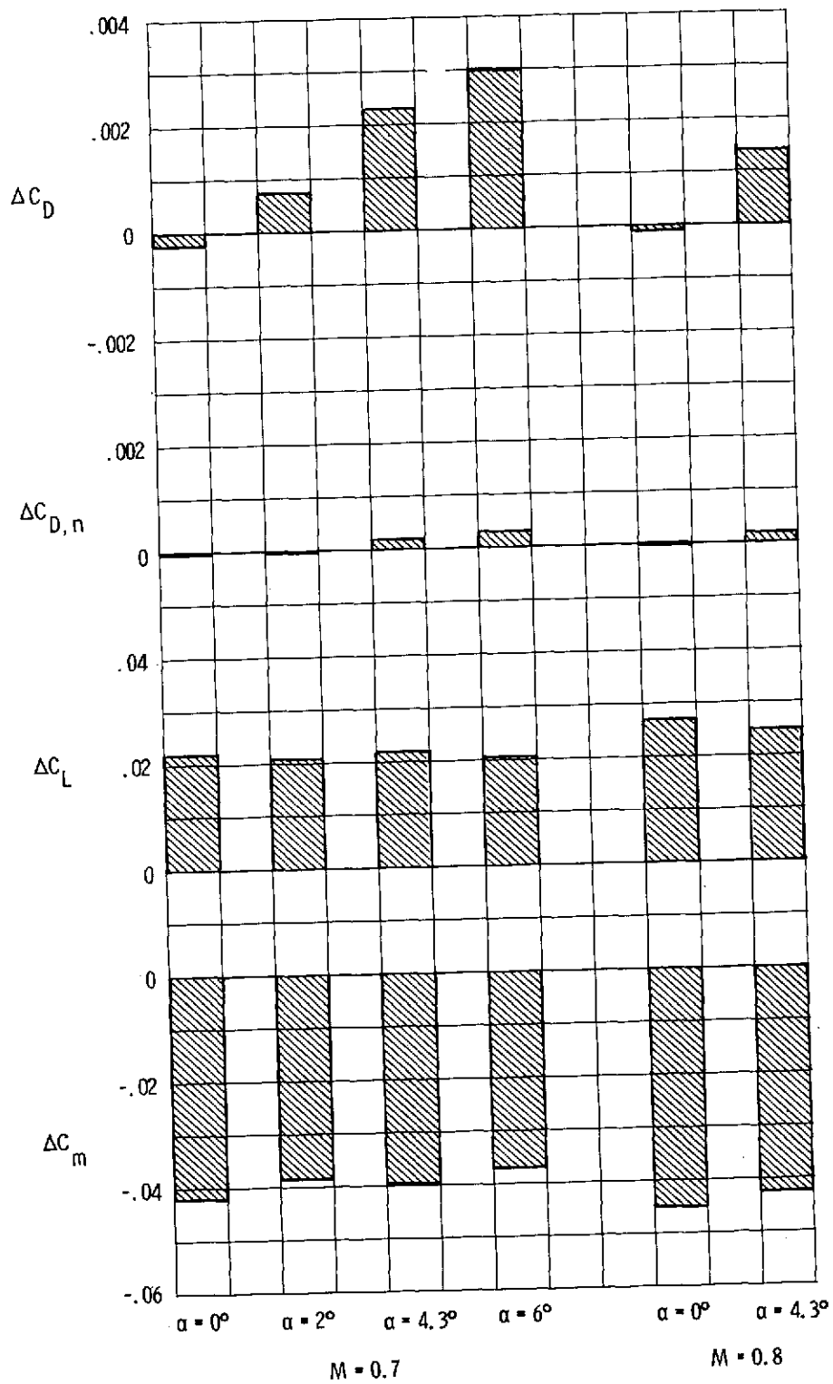
Figure 38.- Increments in afterbody-nozzle aerodynamic characteristics due to deflecting horizontal tails from 0^\circ to +2^\circ with type A cruise nozzles and interfering 2.
