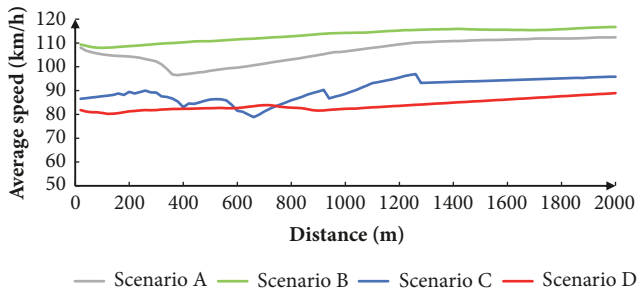
FIGURE 8: Distribution of average speed under different scenarios.
