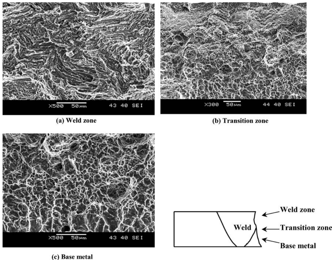
Figure 8 Fracture surfaces at various locations of a weld made with 10% oxygen content.
