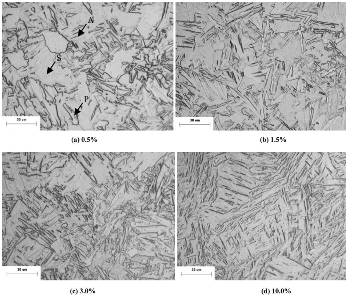
Figure 3 Cross sections of welds made with various oxygen content in argon shielding gas.
