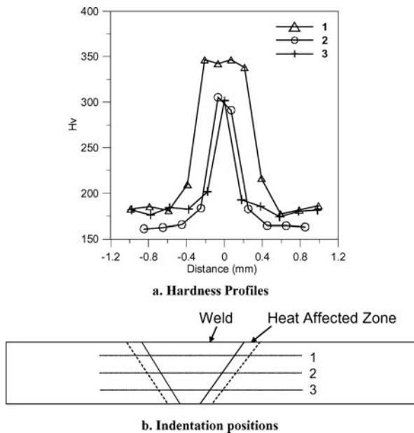
Figure 4 Hardness profiles along the cross section of weld made with 10% oxygen content.
