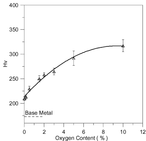
Figure 5 Weld hardness versus oxygen content in argon shielding gas.
