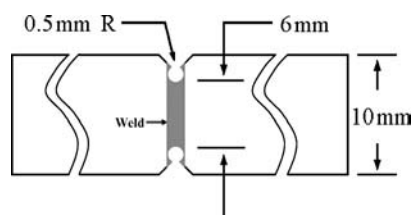
Figure 1 Design of tensile specimen.
