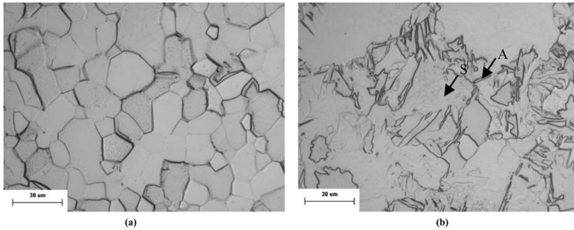
Figure 2 Cross sections of (a) base metal and (b) weld made with pure argon shielding gas.
