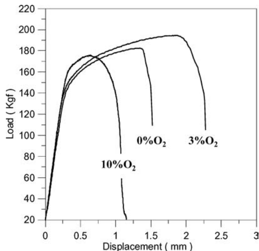
Figure 7 Load-displacement curves for welds made with various oxygen contents.
