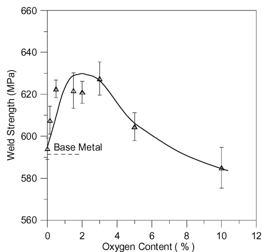
Figure 6 Weld tensile strength versus oxygen content in argon shielding gas.
