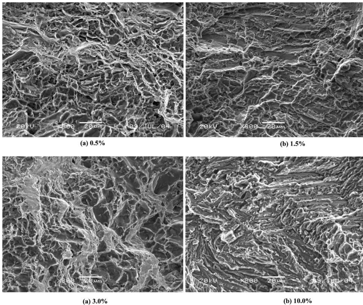
Figure 9 Fracture surfaces of welds made with various oxygen content in argon shielding gas.
