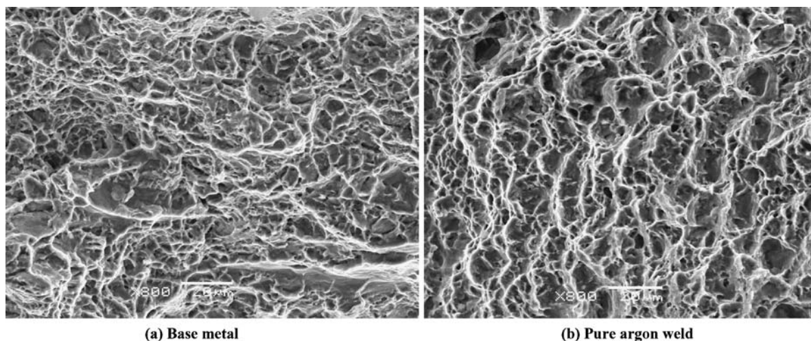
Figure 10 Fracture surfaces of (a) base metal and (b) weld made with pure argon shielding gas.
