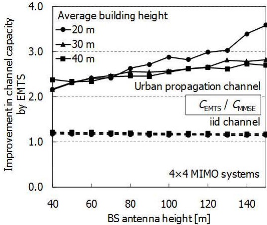
Fig.3: Improvement in channel capacity by EMTS.
