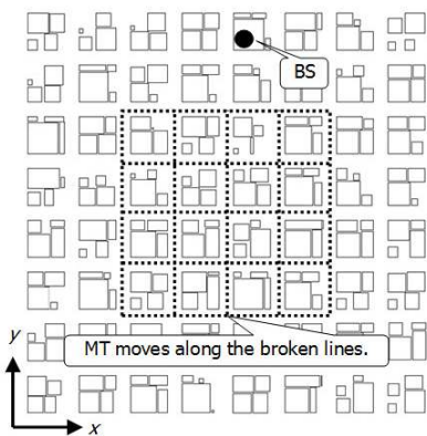
Fig.1: Urban propagation model.
