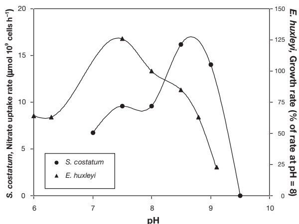
Fig. 13. Skeletonema costatum . Nitrate uptake rate (Thoresen et al. 1984). Emiliania huxleyi . Growth rate relative to growth rate at pH 8 (Paasche 1964). Curve fits are interpolations
