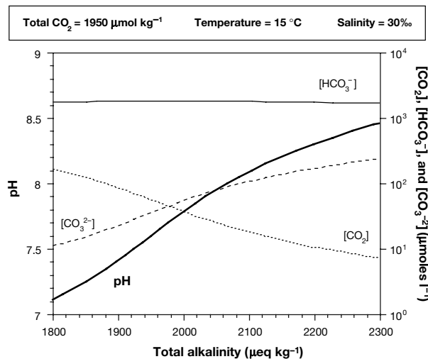
Fig. 4. Alkalinity vs pH and CO 2 species. See Fig. 3 legend
