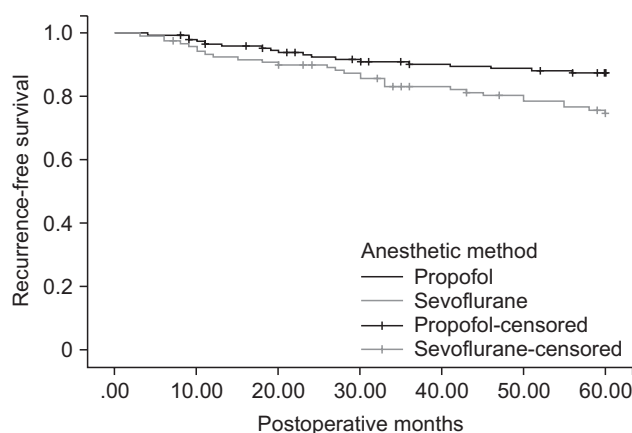
Fig. 2. Kaplan-Meier recurrence-free survival estimated for 325 patients receiving propofol-based total intravenous anesthesia (173) and sevoflurane-based anesthesia (152). Univariate analysis by log-rank test ( P = 0.037 ).
