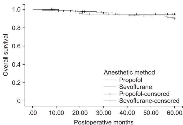
Fig. 1. Kaplan-Meier overall survival estimated for 325 patients receiving propofol-based total intravenous anesthesia (173) and sevoflurane-based anesthesia (152). Univariate analysis by log-rank test ( P = 0.383 ).
