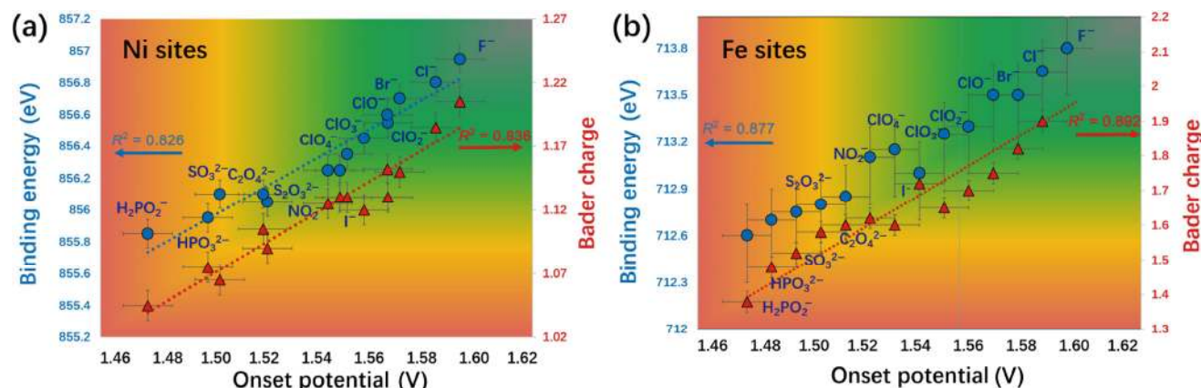
Figure 8 Binding energy and Bader charge of (a) Ni and (b) Fe sites as a function of the experimentally measured onset potential in as-prepared LDHs (●: Binding energy; ▲: Bader charge).
