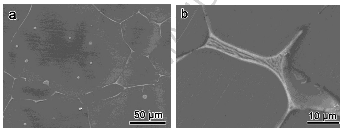
Figure 2 (a) SEM micrograph of the as-cast alloy; (b) SEM micrograph showing the eutectic product along the grain boundaries.
