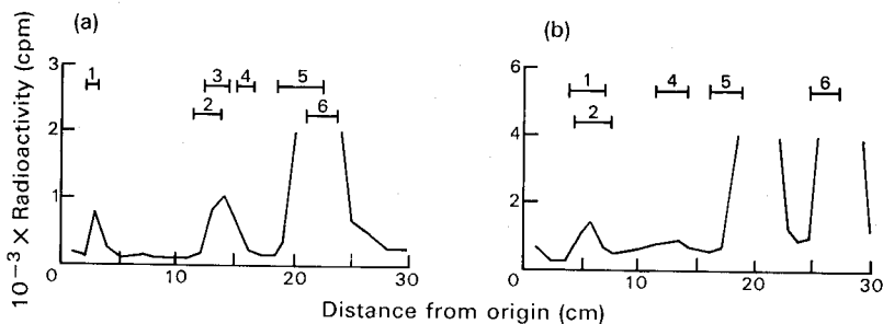
Fig. 5. Chromatogram profiles showing the separation of ^{14}\text{C} -labelled intermediates of chitin synthesis. Extracts were prepared from larval integuments following incubation with ^{14}\text{C} -labelled substrates. (a) ^{14}\text{C} -labelled NAG as substrate; chromatogram developed with the GW-3 solvent system. (b) ^{14}\text{C} -labelled Gm as substrate; chromatogram developed with pyridine-propan-1-ol-acetic acid-water. Descending paper chromatography was used. After development with the solvent, chromatograms were cut into 1 cm pieces and the level of radioactivity in each piece was determined. Positions occupied by marker compounds are shown above the profile: 1, UDPAG; 2, Gm-6-P; 3, NAG-1-P; 4, NAG-6-P; 5, NAG; 6, Gm.
