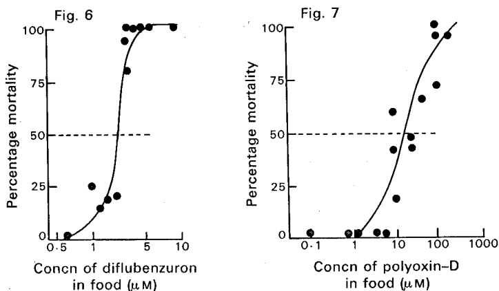
Figs 6 and 7. Log dosage–percentage mortality curve for second-instar larvae fed with diflubenzuron (Fig. 6) and with polyoxin-D (Fig. 7).
