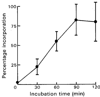
Fig. 2. Incorporation of ^{14}\text{C} -labelled NAG into chitin by isolated larval integuments. The data represent the percentages of maximum incorporations for each experiment and 100% incorporations range from 2–5% of input radioactivity. Each point is the mean of five separate determinations and the vertical bars show \pm 1 s.d.
