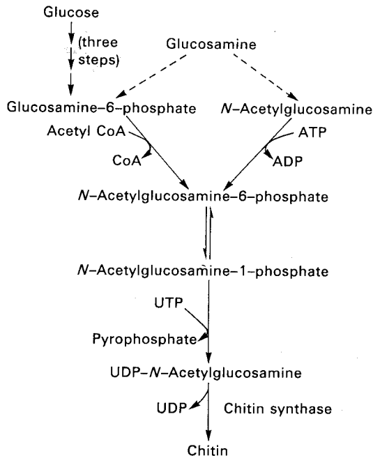
Fig. 1. Postulated pathways for chitin biosynthesis in arthropods (from Gwinn and Stevenson 1973). The broken arrows indicate two possible entry points for glucosamine.
