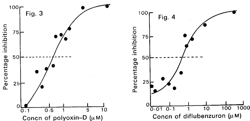
Figs 3 and 4. Inhibition of chitin synthesis in isolated larval integuments by polyoxin-D (Fig. 3) and by diflubenzuron (Fig. 4). Points (means of duplicates) are expressed as percentages of control incorporations obtained using the same batch of larvae. Inhibitor concentrations are on a logarithmic scale.
