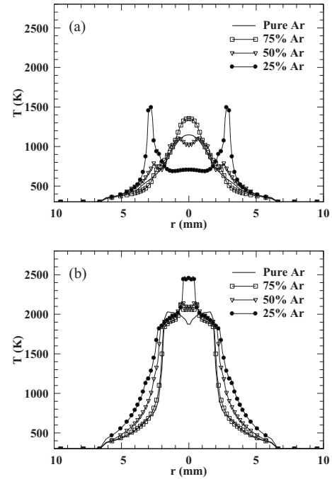
FIG. 12. The metal temperature along the workpiece surface at different instants corresponding to the cases shown in Fig. 3: (a) the first column and (b) the fifth column.
