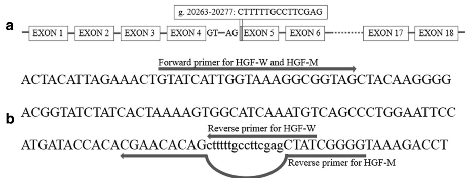
Fig. 3 Alternative splicing of bovine HGF gene. a The genomic location of splicing fragment ( gray region ) in HGF-M was compared to HGF-W. Boxes show the exons and lines represents introns. Dashed line indicating the partial genomic structures are not listed. b Positions of primers for detecting the HGF-W and HGF-M mRNA expression level. Lower cases show the splicing fragment sequence. The bow line indicates that the reverse primer for HGF-M skips the splicing fragment
