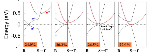
FIG. 2: (color online) Calculated band structures of the strained graphene around the S point with a Z -strain of 24.0%, 26.2%, 26.5% and 27.0% (from left to right panels), respectively.
