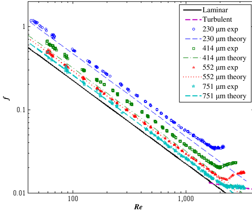
Figure 41. Experimental and Theoretical Friction Factor vs. Reynolds Number, \lambda/h = 3 b = 230, 414, 552, \text{ and } 751 \mu\text{m}
