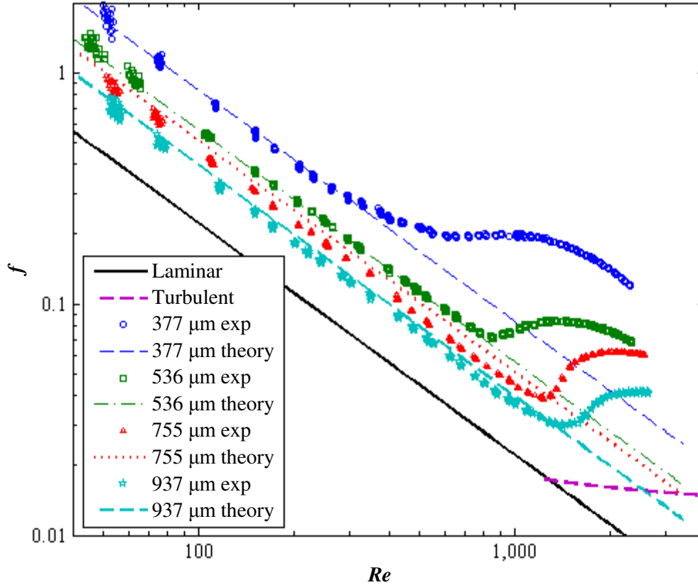
Figure 42. Experimental and Theoretical Friction Factor vs. Reynolds Number, \lambda/h = 2 b = 377, 536, 755, and 937 \mu\text{m}
