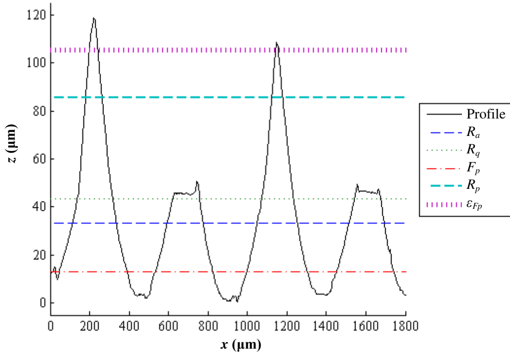
Figure 4. Profilometer Data for 815 \mu\text{m} Pitch Saw-tooth Roughness Profile with Amplitude Parameters and Constricted Parameter, \varepsilon_{Fp}
