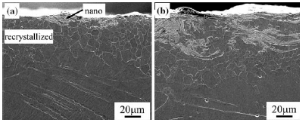
Figure 10. Microstructure of shot peened Fe-3.29Si after annealing at 873 K for 3.6 ks: (a) 3,000%, (b) 10,000% [19].
