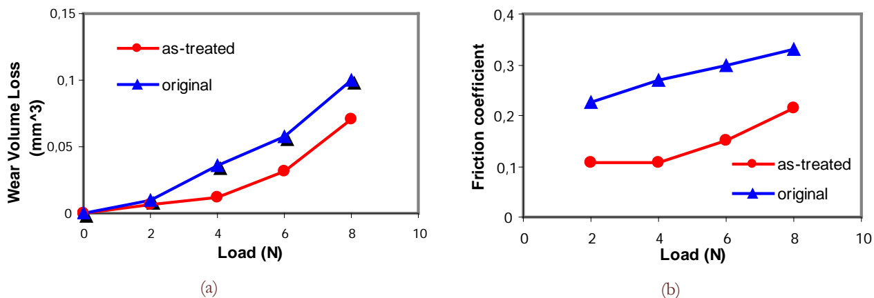
Figure 8. Variations of the wear volume loss with load (a) and variations of the coefficient of friction with load (b) for the SMAT and the original low-carbon steel samples [73].
