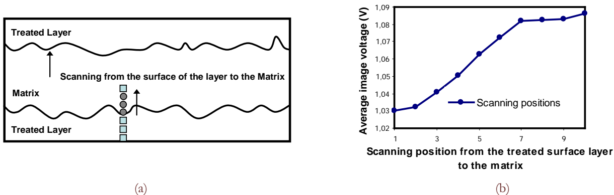
Figure 12: (a) Schematic diagram of the scanning positions from the surface layer to the matrix on the cross-sectional surface. (b) Variation in average image voltage while scanning from the treated surface layer to the matrix as indicated in (a) [97].
