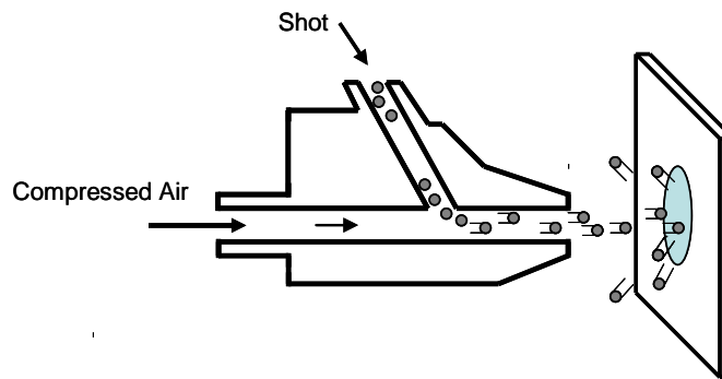
Figure 3: Schematic illustration showing the equipment of ABSP.
