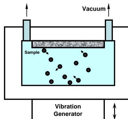
Figure 4: Sketch of SMAT
