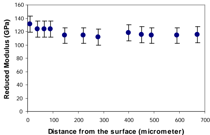
Figure 7: Reduced modulus versus the distance for the sample surface for a load P=10 mN [88].
