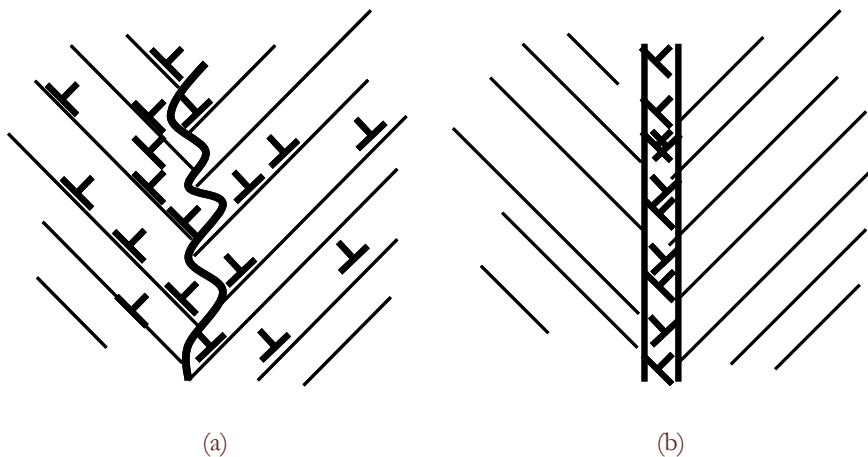
Figure 1: Arrangement of grain boundaries in nanostructured layers: (a) the dislocation structure during SPD processing (b) the dislocation structure after SPD processing leading to formation of non-equilibrium grain boundaries.
