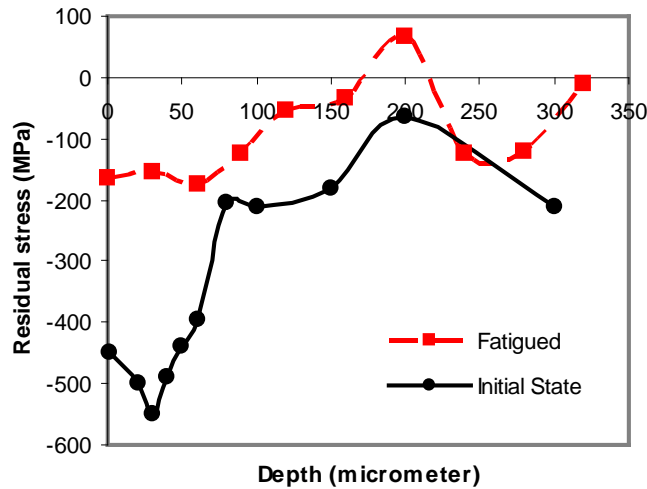
Figure 6: Residual stress depth profiles of shot peened (Almen intensity 0.175 mmA) AISI 304 before and after cyclic loading with \sigma_a = 320 MPa after N_f/2 cycles [62].
