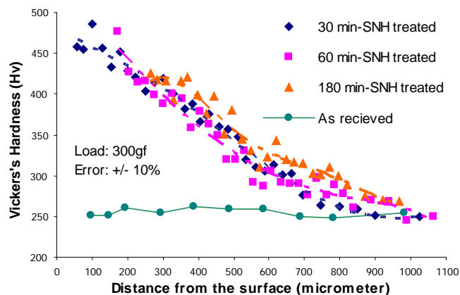
Figure 11: Hardness profile of the samples [80].
