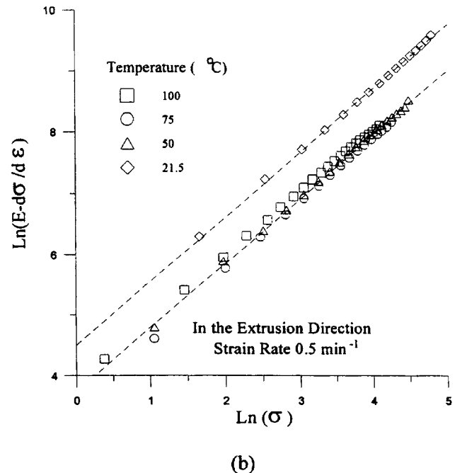
Fig. 7. Plots of \ln(E - d\sigma/d\varepsilon) vs. \ln \sigma for short E-glass fiber reinforced polyamide-6 in the extrusion direction. (a) 0.05 \text{ min}^{-1} , (b) 0.5 \text{ min}^{-1} and (c) 5 \text{ min}^{-1} .
