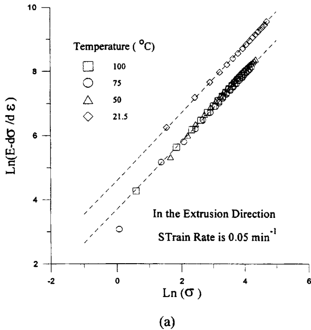
Fig. 7. Plots of \ln(E - d\sigma/d\varepsilon) vs. \ln \sigma for short E-glass fiber reinforced polyamide-6 in the extrusion direction. (a) 0.05 \text{ min}^{-1} , (b) 0.5 \text{ min}^{-1} and (c) 5 \text{ min}^{-1} .
