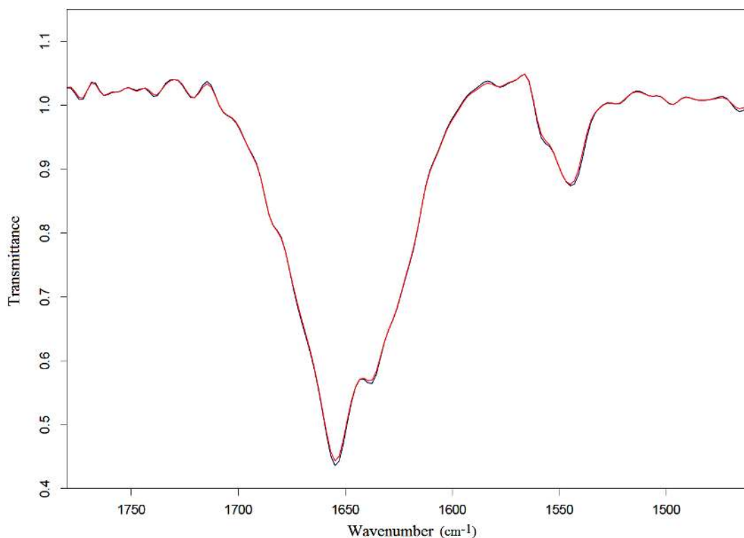
Fig. (4). FSD representative spectra of Amide I and Amide II regions of hemoglobin in NaCl water solution after 3 h of exposure to 1750 MHz mobile phone MWs at the power density of 950 mW/m 2 (red line refers to exposed sample). No appreciable change was observed in this analysis after exposure of hemoglobin samples in NaCl water solution.
