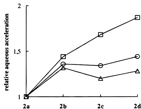
Figure 2. Relative aqueous accelerations ( k_{water}/k_{1-PrOH} ), normalized to the acceleration of the reaction with 2a , for the reactions of 1 (○) and 4 (□) with 2a–d relative to n -hexane, and for the reaction of 6 (△) with 2a–d relative to 1-propanol.
