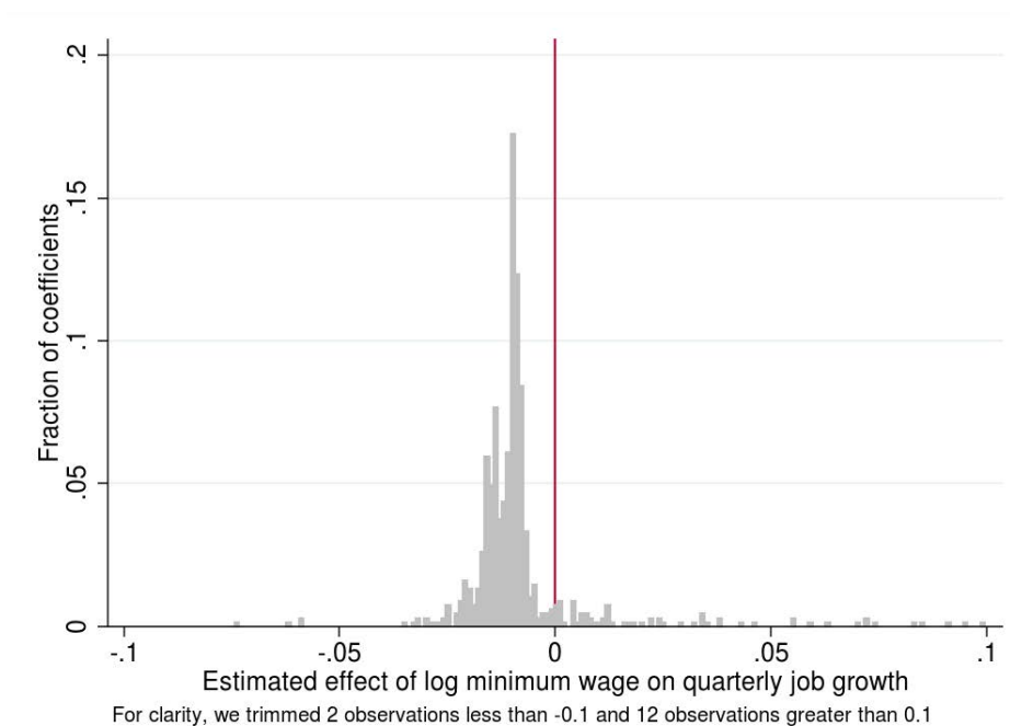
Figure B.2: Distribution of point estimates from subsamples of time-spans in the QCEW
