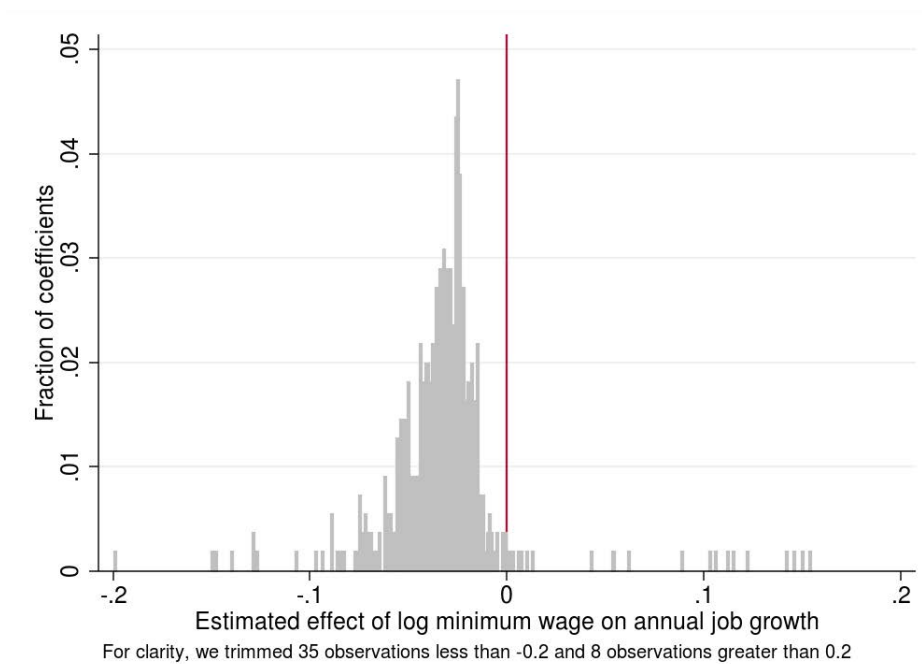
Figure B.1: Distribution of point estimates from subsamples of time-spans in the BDS
