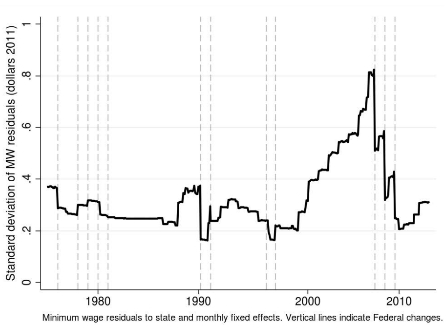
Figure C.5: Standard deviation of residual state real minimum wages (1975-2012)
