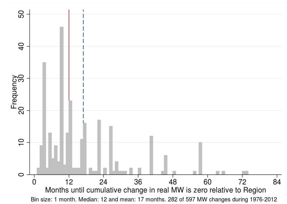
Figure C.11: Erosion of relative increases in minimum wage
