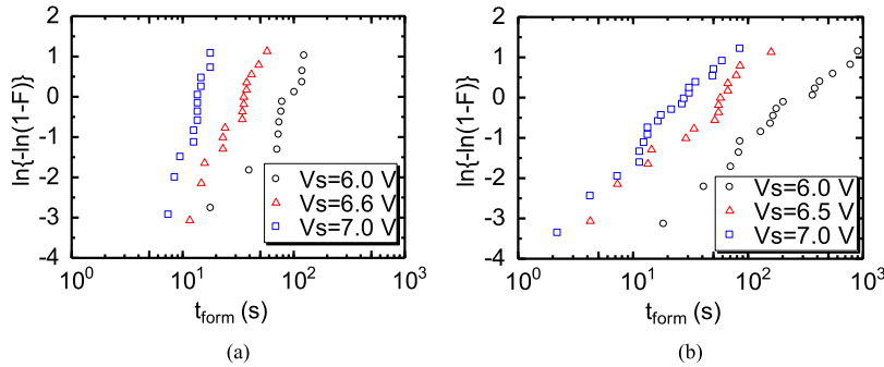
FIG. 9. Dependence of the Weibits of time to forming ( t_{\text{form}} ) on the applied constant voltage ( V_s ) in (a) the SP-Pt samples and (b) the EB-Pt samples.
