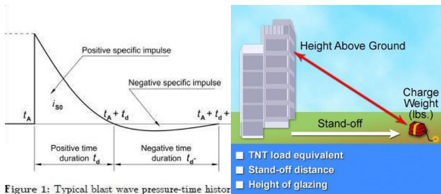
Figure 1: Typical blast wave pressure-time history
