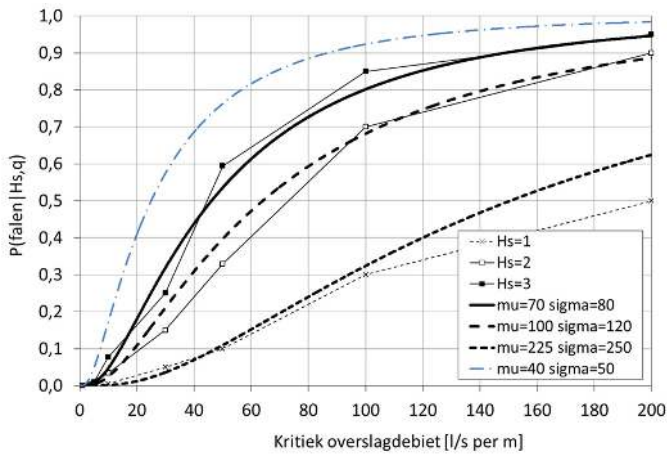
Figure 4.3 Probability distribution of the critical wave overtopping discharge for different significant wave heights including fit-functions (lognormal functions) (RWS et al 2013)
