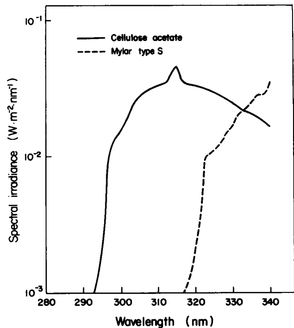
FIG. 1. Unweighted spectral irradiance of FS-40 sunlamps at 0.2 m filtered through either 0.076-mm cellulose acetate or 0.13-mm Mylar filters.
