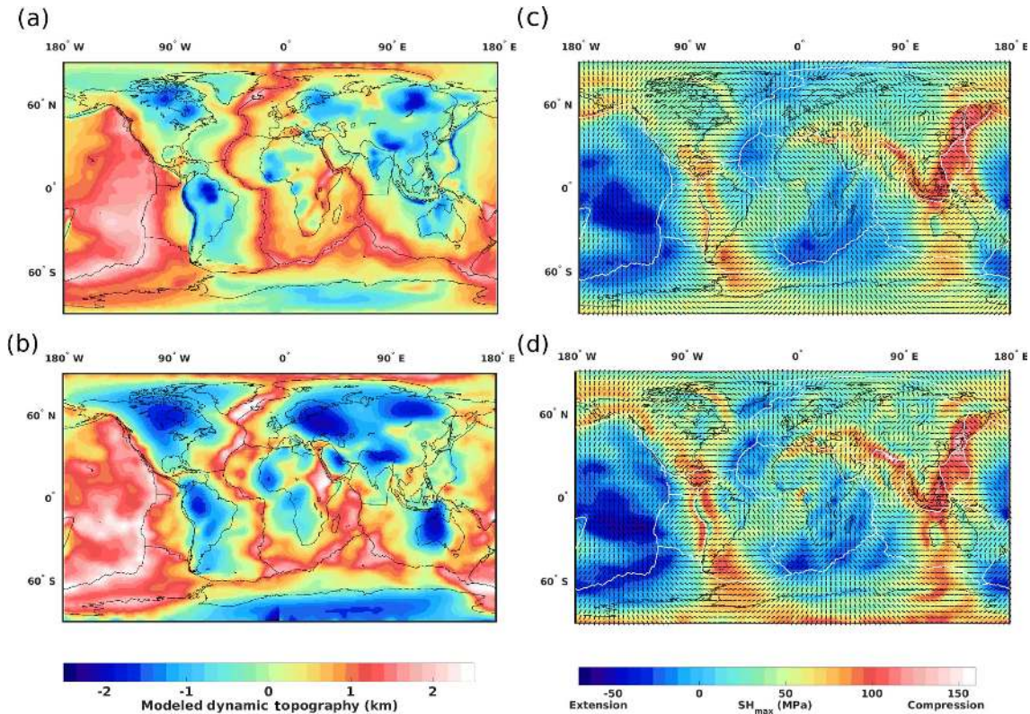
Figure 8. Modeled “dynamic” topography using the upper mantle structure (a) TM1 and (b) TM2 and corresponding SH max prediction with (c) TM1 and (d) TM2. In contrast to Fig. 4, the effect of the crust is not included here.
