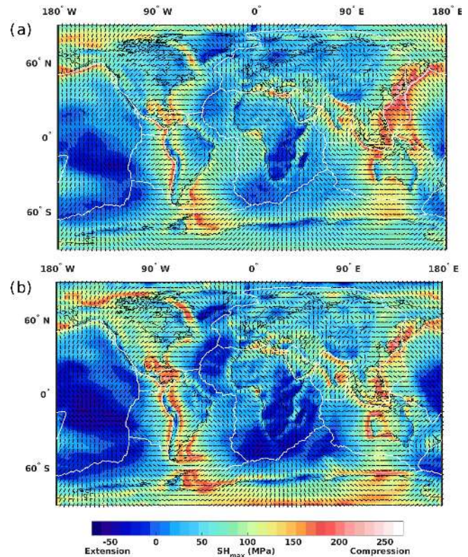
Figure 4. Predictions of the SH_{\max} magnitude and direction from combined contributions due to lower mantle flow and upper mantle from (a) TM1 with crust model and (b) TM2 with crust model beneath air (free surface).
