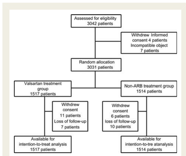
Figure 2 Trial profile.
