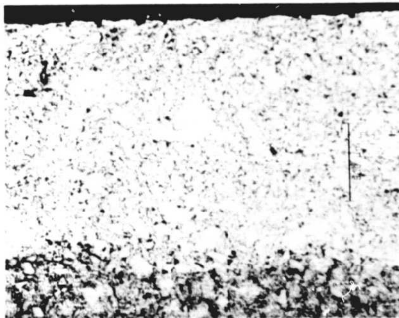
Figure 7 : Photomicrograph of post-sessile drop section of polished Ultracarbon silicon carbide coated graphite after 1 3/4 hour experiment at pO_2 = 10^{-19.9} atm. showing infiltration of silicon below SiC coating.
