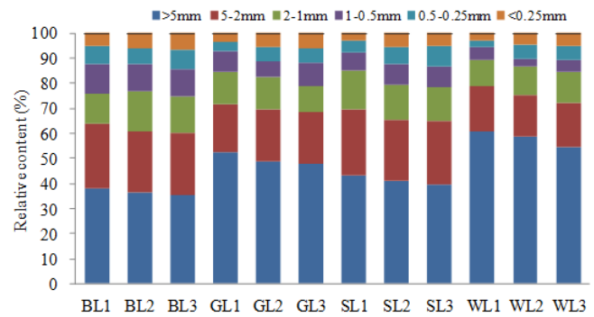
Figure 2. Relative distribution of soil dry aggregates with different sizes under different vegetation types. (BL1, BL2, BL3, GL1, GL2, GL3, SL1, SL2, SL3, WL1, WL2, and WL3 represent 0–20 (1), 20–40 (2), and 40–60 cm (3) soil layers of bare land (BL), grassland (GL), shrubland (SL), and woodland (WL), respectively.)
