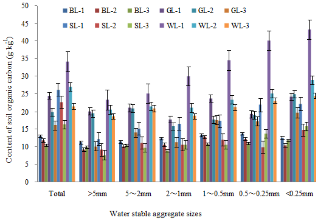
Figure 1. SOC in different water-stable aggregate sizes under different vegetation types (mean \pm SE, n = 3 ). BL1, BL2, BL3, GL1, GL2, GL3, SL1, SL2, SL3, WL1, WL2, and WL3 represent 0–20 (1), 20–40 (2), and 40–60 cm (3) soil layers of bare land (BL), grassland (GL), shrubland (SL), and woodland (WL), respectively).
