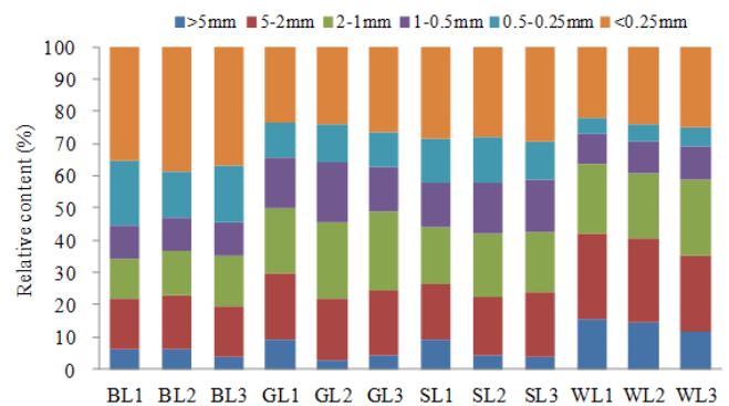
Figure 3. Relative distribution of soil water-stable aggregates with different sizes under different vegetation types (BL1, BL2, BL3, GL1, GL2, GL3, SL1, SL2, SL3, WL1, WL2, and WL3 represent 0–20 (1), 20–40 (2), and 40–60 cm (3) soil layers of bare land (BL), grassland (GL), shrubland (SL), and woodland (WL), respectively.)
