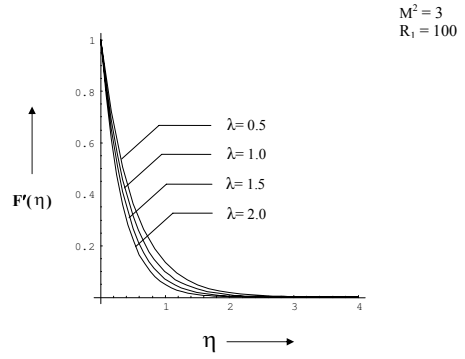
Fig. 4. Dimensionless longitudinal velocity profiles for different \lambda .
