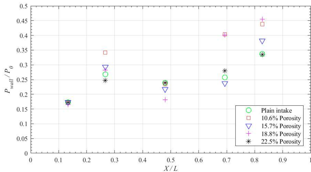
Figure 13. Static pressure variation along the intake-core due to wall ventilation at R_c = 1.19 .
