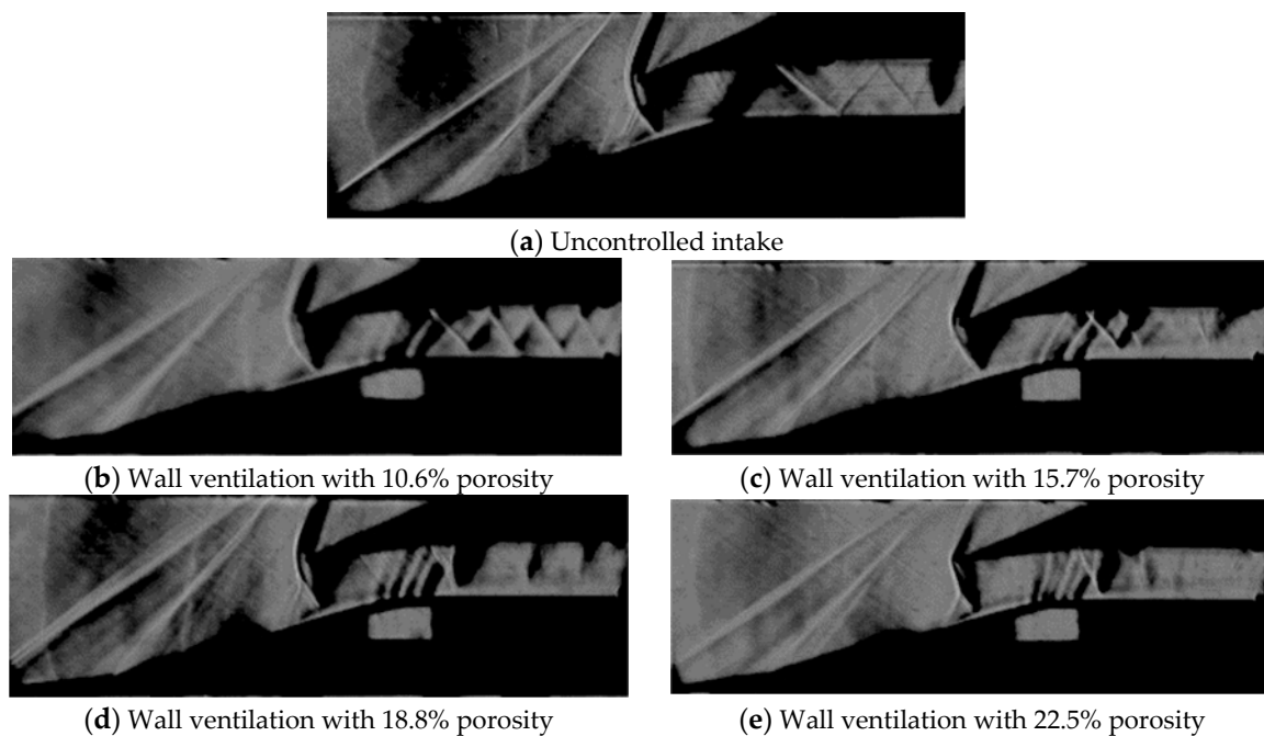
Figure 10. Schlieren view of uncontrolled and wall ventilated intakes at R_c = 1.25 .
