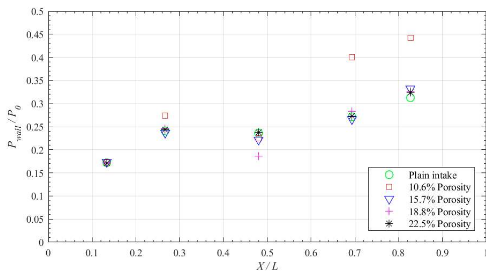
Figure 14. Static pressure variation along the intake-core due to wall ventilation at R_c = 1.22 .
