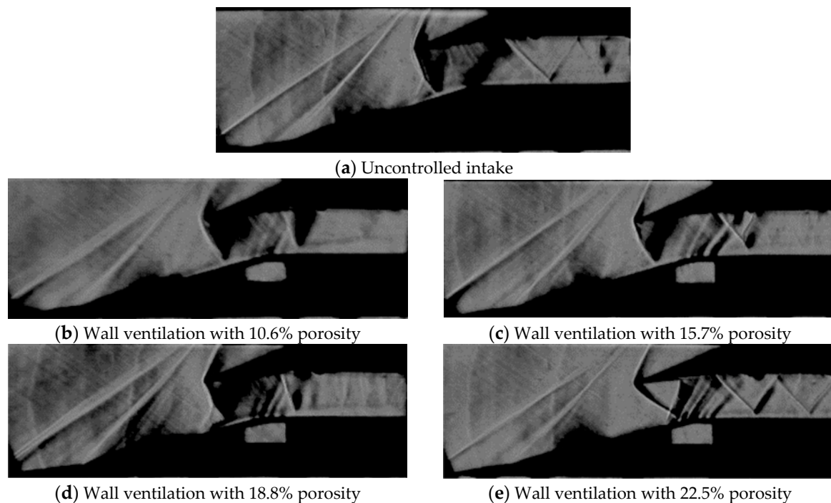
Figure 8. Schlieren view of uncontrolled and wall ventilated intakes at R_c = 1.19 .
