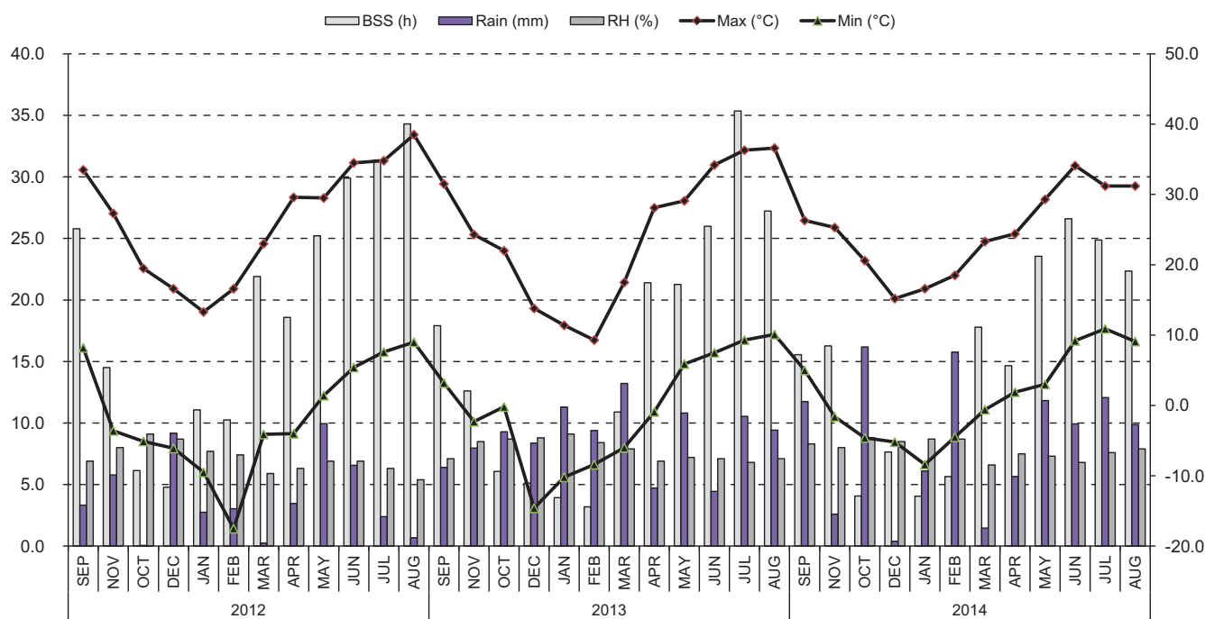
FIGURE 1. Monthly variations in weather parameters: maximum temperature (Max), minimum temperature (Min), relative humidity (RH), rainfall (Rain) and bright sunshine hours (BSS) during 2012, 2013 and 2014 growing seasons.
