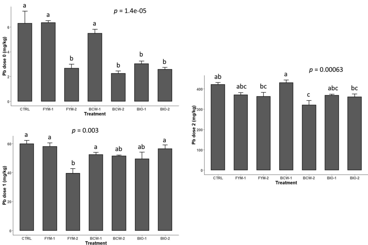
Fig. 2 Concentrations of the bioavailable fractions of Pb in soil contaminated by HMs at dose 0 (a), dose 1 (b) and dose 2 (c) after treatment by different organic materials. Values are treatment means ( \pm se), n = 6 . Bars that do not share a letter are significantly different according to Nemenyi's test for multiple comparisons
