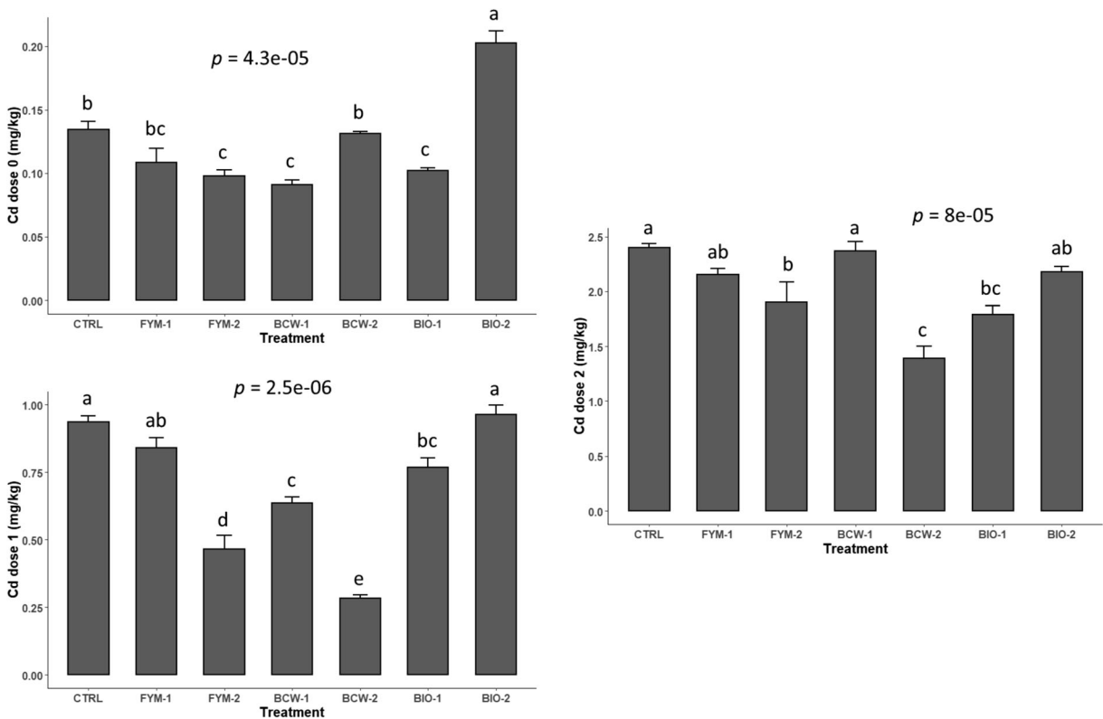
Fig. 1 Concentrations of the bioavailable fractions of Cd in soil contaminated by HMs at dose 0 (a), dose 1 (b) and dose 2 (c) after treatment by different organic materials. Values are treatment means ( \pm se), n = 6 . Bars that do not share a letter are significantly different according to Nemenyi's test for multiple comparisons
