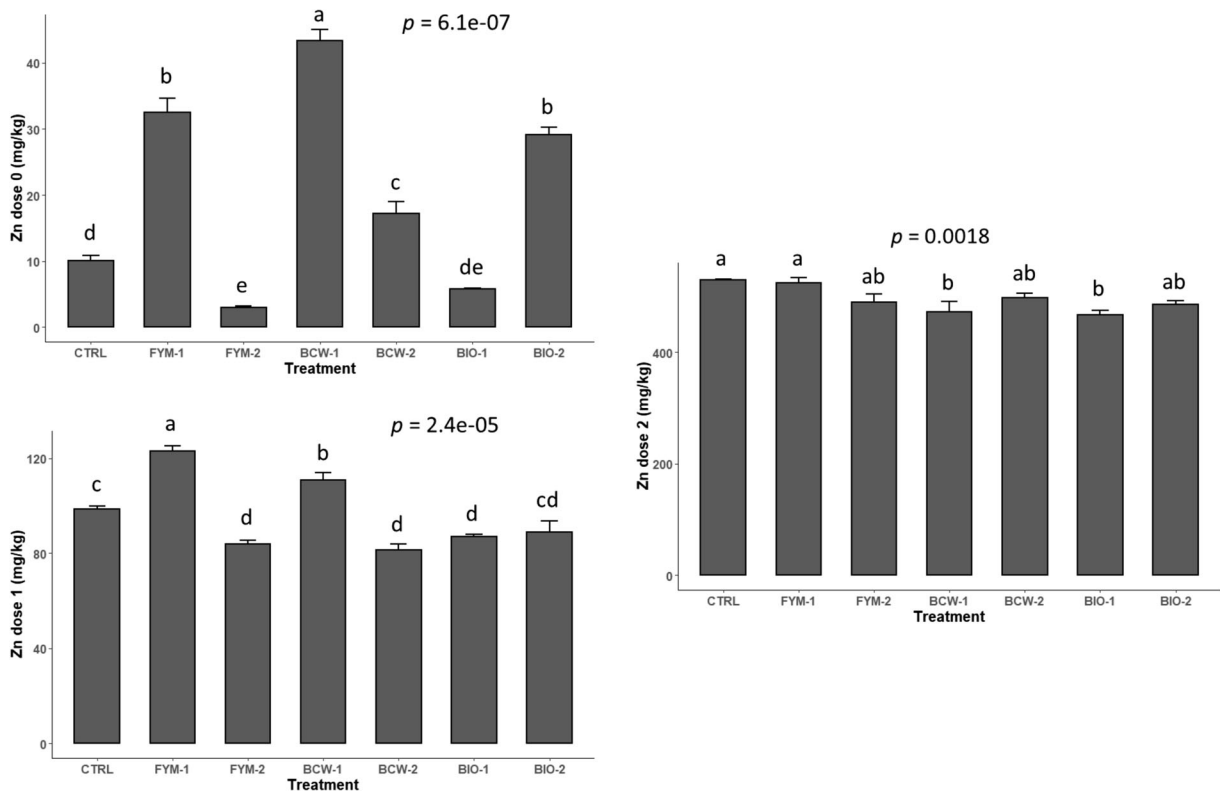
Fig. 3 Concentrations of the bioavailable fractions of Zn in soil contaminated by HMs at dose 0 (a), dose 1 (b) and dose 2 (c) after treatment by different organic materials. Values are treatment means ( \pm se), n = 6 . Bars that do not share a letter are significantly different according to Nemenyi's test for multiple comparisons
