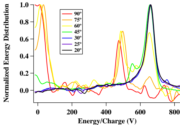
Figure 6. Normalized Voltage Distribution Function for Operation Point 12
