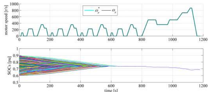
Fig. 8: The motor speed and SOC of battery cells.
