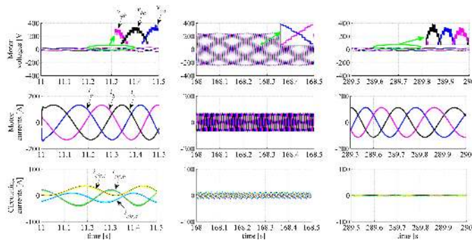
Fig. 7: The motor line voltages and currents, and the converter circulating currents.
