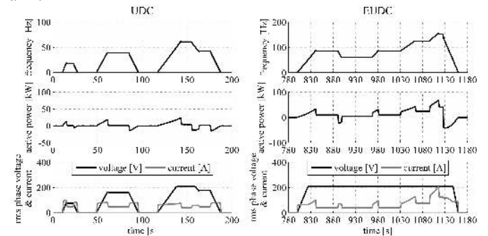
Fig. 9: The motor electric active power, voltage and current.
