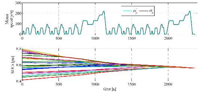
Fig. 12: The motor speed, and SOC's of battery cells.
