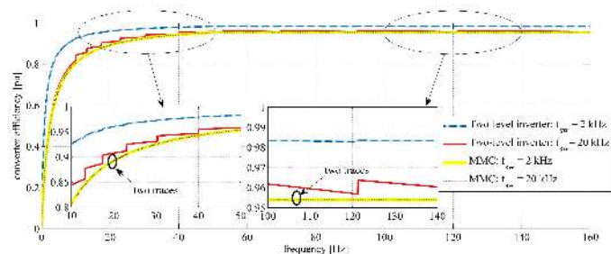
Fig. 6: The efficiency for both topologies versus frequency at full-load current.
