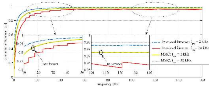
Fig. 5: The efficiency for both topologies versus frequency at half full-load current.
