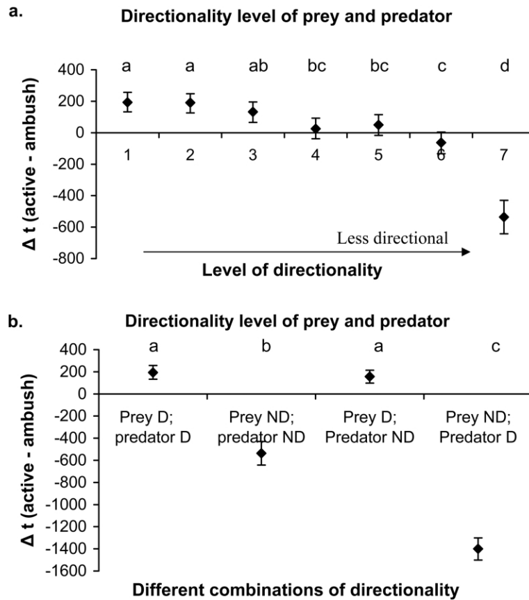
Figure 4: Relationship between the relative time to capture (active predator t_{\text{capture}} – ambush predator t_{\text{capture}} ) and movement directionality (as shown in table 1). In most pairwise tests, P < .05 ( P values were estimated using bootstrap tests). a , Decreased directionality results in an increase in the relative success of the active predator ( P < .05 for most cases). b , Different combinations of prey and predator movement directionality: D = directional movement; ND = nondirectional movement. When prey moved directionally, encounter rates were not significantly influenced by predator movement directionality. In other words, when prey moves nondirectionally, the predator would do better to adopt a directional form of movement. Different letters indicate significant differences ( P < .05 ).
