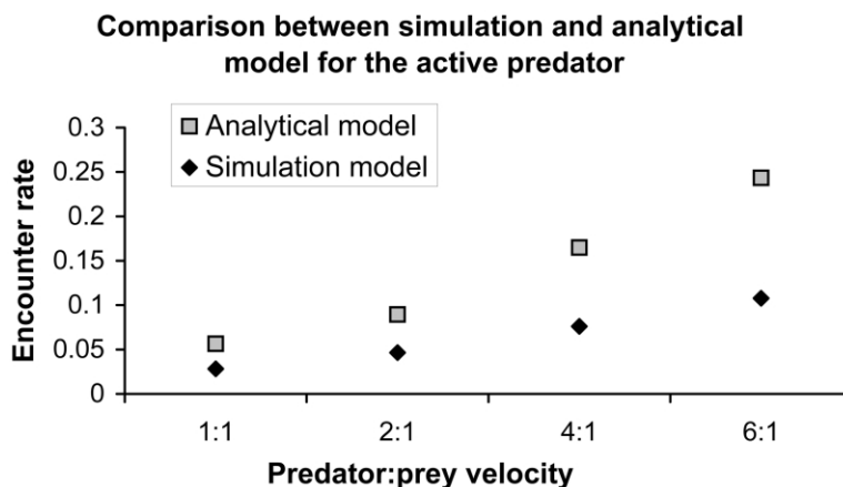
Figure 3: Positive correlation between predator velocity and encounter rates ( t_{\text{capture}}^{-1} ). Simulation results were qualitatively similar to an analytical model derived by Werner and Anholt (1993). We used an arena of 20 \times 20 squares and assigned nondirectional movement to both the active predator and 12 prey items.
