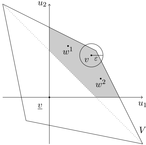
FIGURE 4. Illustration of Theorem 4.1 for n = 2 . The shaded area is \mathbf{co}(\mathcal{P}(V)) , which is contained in the limit set of PBE payoffs. w^1 and w^2 are used to construct player-specific punishments.
