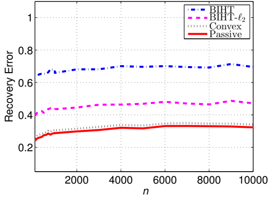
Figure 3. The recovery error of each algorithm versus the dimensionality n , when s = 10 and m = 1000 .
