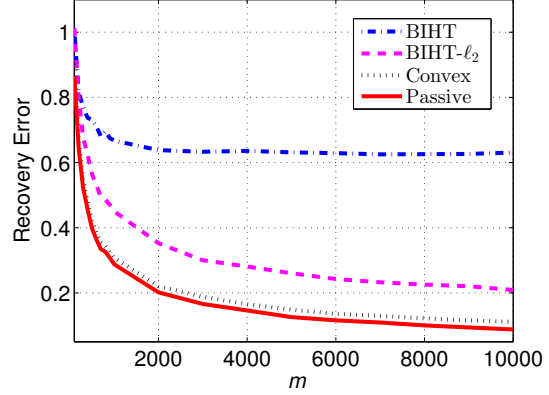
Figure 2. The recovery error of each algorithm versus the number of measurements m , when s = 10 and n = 1000 .
