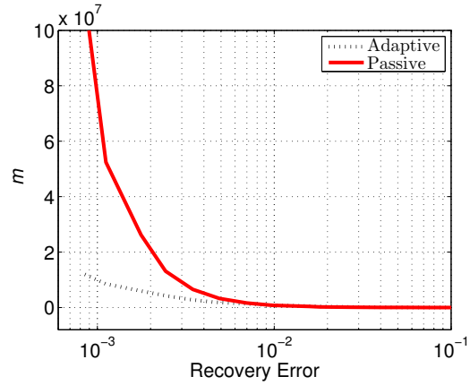
Figure 4. The number of measurements required by the passive and adaptive algorithms versus the recovery error, when s = 10 and n = 1000 .
