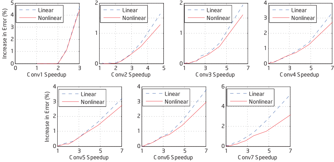
Figure 4. Linear vs. Nonlinear: single-layer performance of accelerating Conv1 to Conv7. The speedup ratios are computed by the theoretical complexity, but is nearly the same as the actual speedup ratios in our CPU/GPU implementation. The error rates are top-5 single-view, and shown as the increase of error rates compared with no approximation ( smaller is better ).
