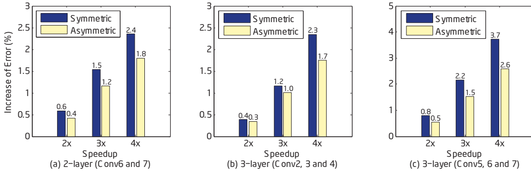
Figure 5. Symmetric vs. Asymmetric: the cases of 2-layer and 3-layer approximation. The speedup is computed by the complexity of the layers approximated. (a) Approximation of Conv6 & 7. (b) Approximation of Conv2, 3 & 4. (c) Approximation of Conv5, 6 & 7.
