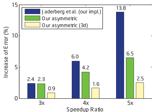
Figure 6. Comparisons with Jaderberg et al. 's spatial decomposition method [10]. The error rates are top-5 single-view, and shown as the increase of error rates compared with no approximation ( smaller is better ).
