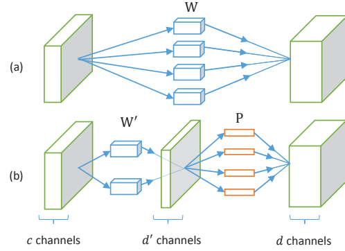
Figure 1. Illustration of the approximation. (a) An original layer with complexity O(dk^2c) . (b) An approximated layer with complexity reduced to O(d'k^2c) + O(dd') .
