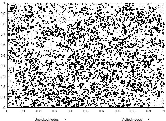
Figure 2: An example of random walk that covers 80% of a random network with 4096 nodes
