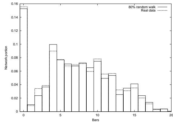
Figure 12: Comparing the histogram founded by the 80% random walk on the graph and the histogram of the real data from Figure 11
