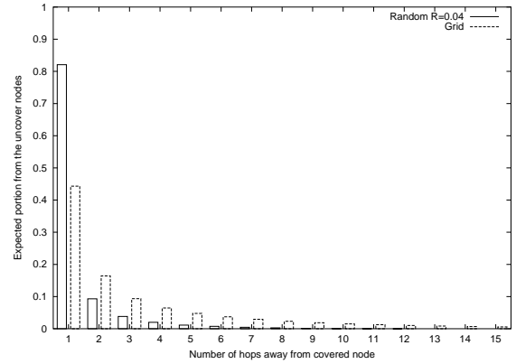
Figure 9: Histogram of the min distance of uncovered nodes from visited nodes after 80% of the network was covered. n=4096
