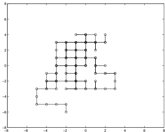
Figure 1: An example of short random walk on a grid starting at (0, 0)
