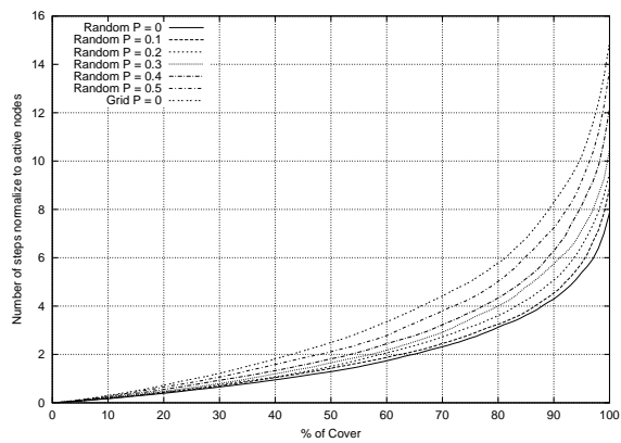
Figure 6: The Partial Cover time required when the probability p of each node to fail is increasing. The result are for 4096 nodes networks
