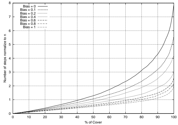
Figure 4: Partial Cover Time in random walks with increasing bias on random network
