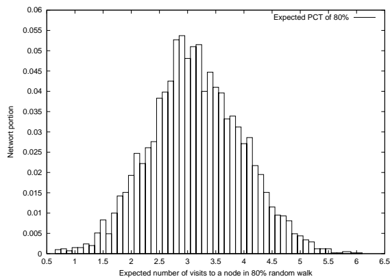
Figure 13: Histogram of the expected number of visits to a node in a 80% cover random walk
