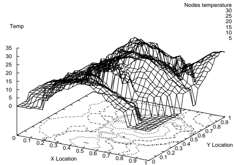
Figure 11: An example of the temperature in an area with six random light sources
