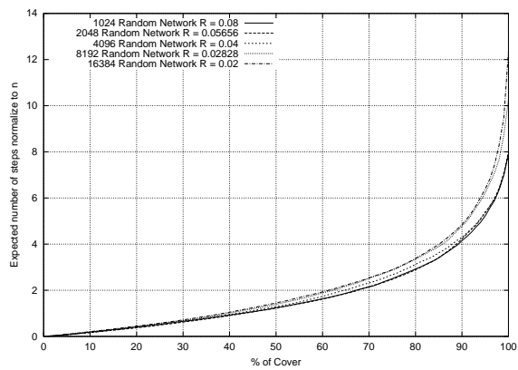
Figure 14: Partial Cover time in increasing size of random network with same density
