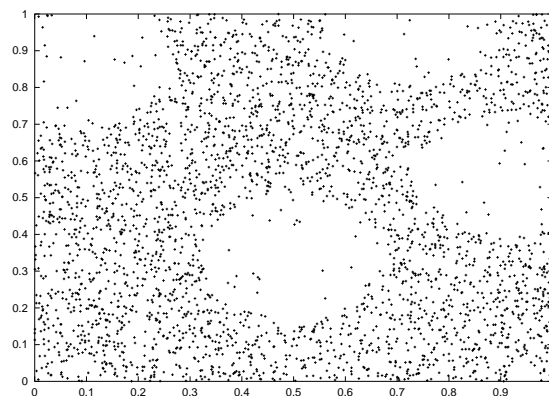
Figure 7: An example of a 4096 random network with 4 disaster areas. We can see the creation of bottlenecks
