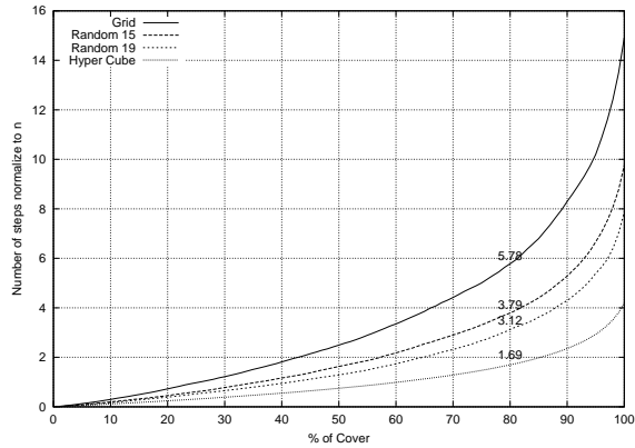
Figure 3: The Partial Cover time progress in four network of size 4096
