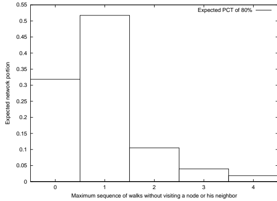
Figure 10: Histogram of the maximum number of consecutive runs without a node or his neighbor in 100 runs of 80% cover
