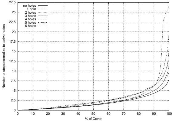
Figure 8: The Partial Cover time required when we increase the number of disaster areas in the network
